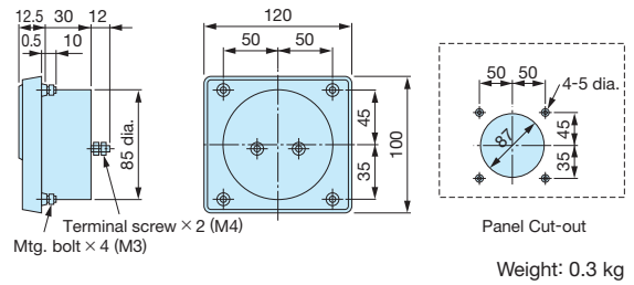
Dimensions (mm)
