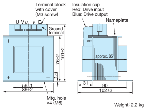
Dimensions (mm)
